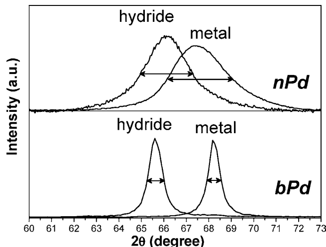
Figure 4. Comparison of the (220) diffraction peak for the metal and hydride phases of nPd (top) and bPd (bottom). The diffraction patterns of nPd correspond to those measured at 0 and 10 kPa hydrogen pressure in Figure 3.
